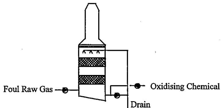
FIGURE 2 Gas Scrubber
