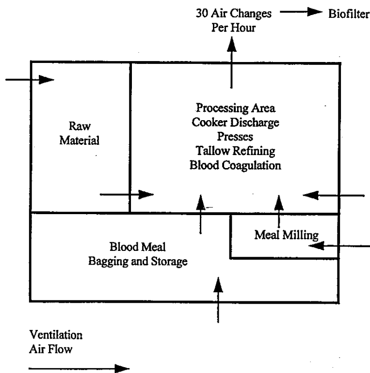
FIGURE 1 Rendering Plant Layout and Ventilation
